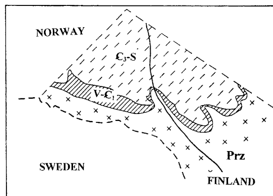
Fig. 1. The most important localities of the Dividal Group on the Scandinavian Peninsula (above): 1, Laisvall-Storuman; 2, Torneträsk; 3, Kilpisjärvi; 4, Avevagge; 5, Halkkavarre; 6, Finnmark. A schematic geological map of the Kilpisjärvi region (below). Striped area shows the outcrop of the Dividal Group.
