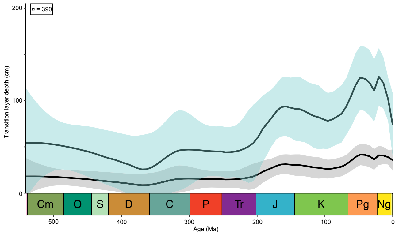
Fig. 4. Transition layer depth over the Phanerozoic. Gray lower curve reflects data with a lower-bound decompaction factor of 1.0 applied; green upper curve reflects data with an upper-bound decompaction factor of 3.0 applied. Curves produced by LOESS smoothing model with \alpha = 0.3 . Shaded areas are 95% confidence intervals. Geological timescale visualized using the R package deptime (v1.1.1) (114).
