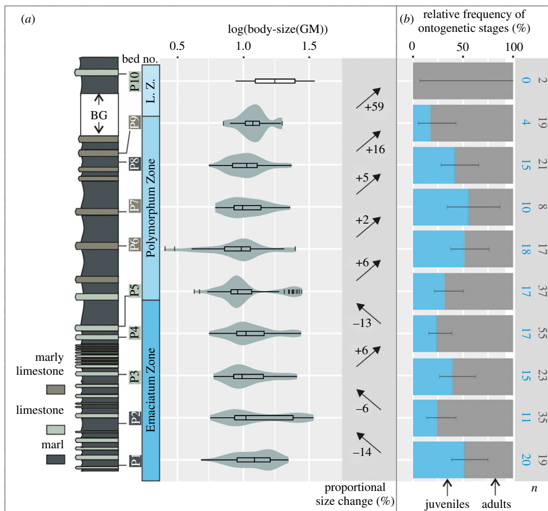
Figure 5. (a) Lithology, belemnite body-size variation (violin plots) and proportional body-size change across the studied interval in Peniche. (b) Relative frequency of ontogenetic stages at the assemblage scale across the studied interval in Peniche. Note that the stratigraphic log is not drawn to scale, for real thickness of beds, see figure 1. The error bars correspond to the 95% confidence interval of the juveniles and adults ratio. BG, belemnite gap; GM, geometric mean; n , sample size.
