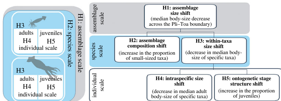
Figure 2. Conceptual scheme depicting the tested hypotheses regarding the mechanisms behind belemnite body-size reduction, at different palaeobiological scales of organization.
