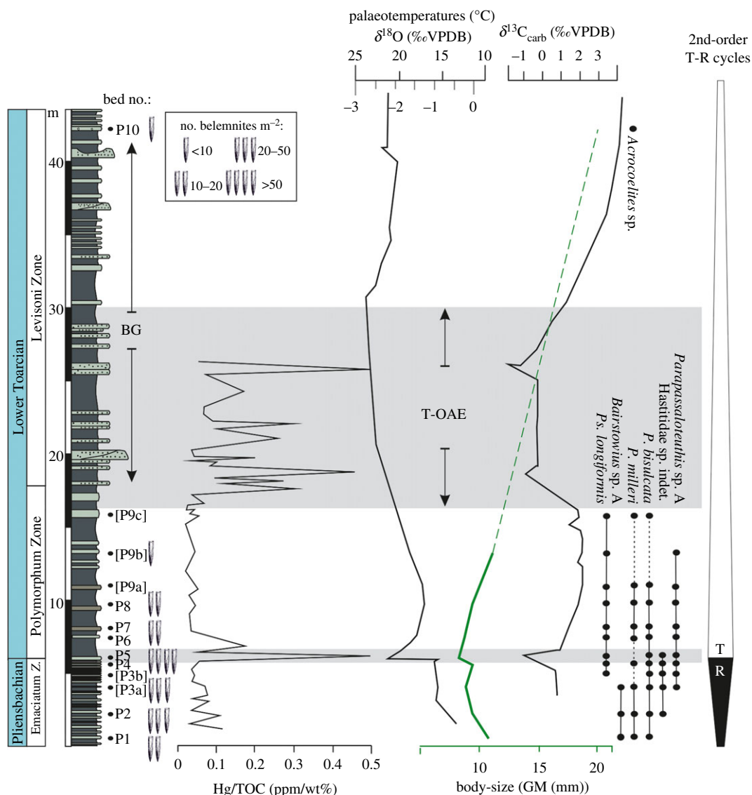
Figure 1. Variation of belemnite body-size (GM, assemblage scale), absolute abundance (no. belemnites \text{m}^{-2} ) and stratigraphic ranges of species, compared with the variation of the analysed geologic proxies (mercury concentration, Hg/TOC [20], carbon and oxygen isotopes, \delta^{13}\text{C}_{\text{carb}} and \delta^{18}\text{O} [21,22]) and sequence stratigraphy data [23] from the Upper Pliensbachian–Lower Toarcian of Peniche. The shaded area highlights the Pli–Toa boundary event. The bed numbers in square brackets correspond to the beds that were merged due to sample size constraints, regarding the belemnite body-size analysis. See electronic supplementary material (figure S2) for details on belemnite abundance. See figure 5 for more information on lithology. Ammonite Zones: Emaciatum Zone, Emaciatoceras emaciatum ; Polymorphum Zone, Dactyloceras polymorphum ; Levisoni Zone, Hildaites levisoni . BG, belemnite gap; GM, geometric mean; T, transgressive; R, regressive.
