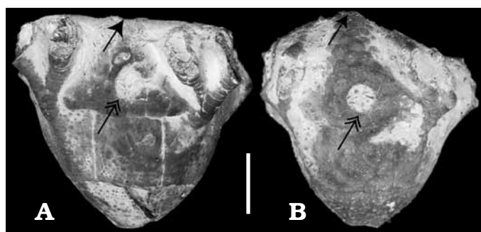
Fig. 1. Specimens of Arthroacantha carpenteri (Hinde, 1885) with drillholes. Each photograph displays the anal interray, position of the anal vent (single arrowheads), and the location of platyceratid drillholes (double arrowheads); scale bar 1 cm. Note the presence of a reaction rim surrounding the drillhole and underdeveloped spine facets below it. Specimens are deposited at the University of Michigan Museum of Paleontology (UMMP). A. UMMP 73711. B. UMMP 73712.
