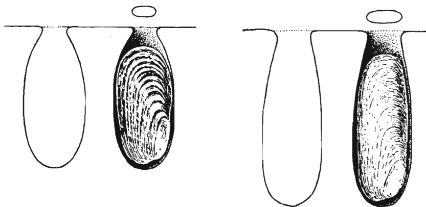
Fig. 1. Borehole of Lithophaga lycetti (Whiteaves) in longitudinal section and two morphologically different specimens inside their boreholes.
