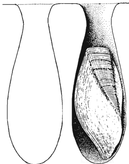
Fig. 7. Borehole of Spengleria recondita (Phillips) in longitudinal section and the shell inside of the borehole; calcareous lining not marked.
