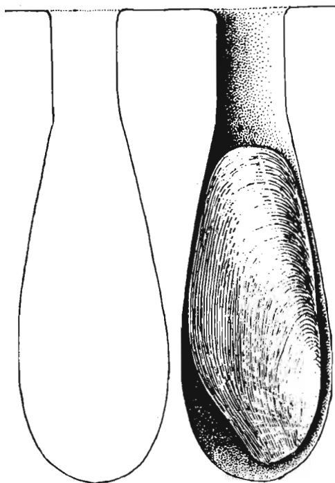
Fig. 10. Borehole of Gastrochaena ( G. ) cf. deshayesea Buvignier in a longitudinal section and shell inside the borehole.
