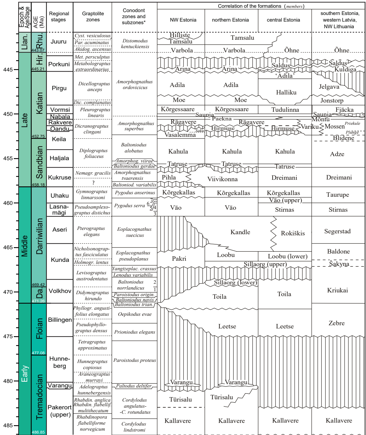
Fig. 4. Ordovician stratigraphy of Estonia. Graptolite zonation according to Kaljo & Vingissaar 1969; Kaljo et al. 1986; Männil 1976; Resheniya... 1987; Männil & Meidla 1994; Nölvak et al. 2006; conodont zones according to Männil in Nölvak et al. 2006; Paiste et al. 2020, 2022 and Meidla et al. 2023. Numbers in the column of the conodont zonation correspond to the conodont subzones as follows: subzones of the Baltoniodus norrandicus Zone: 1 – Trapezognathus quadrangulum Subzone, 2 – Lenodus antivariabilis Subzone; subzones of the Pygodus serra Zone: 3 – Eoplacognathus foliaceus Subzone, 4 – Eoplacognathus reclinator Subzone, 5 – Eoplacognathus robustus Subzone, 6 – Eoplacognathus protoamosus Subzone, 7 – Eoplacognathus lindstroemi Subzone. Abbreviations: Llan., Llandovery; Da., Darriwilian; Hir., Hirnantian; Rhu., Rhuddanian; Cyst., Cystograptus; Par., Parakidograptus; Met., Metabolograptus; Dic., Dicellograptus; Nemagr., Nemagraptus; Holmogr., Holmograptus; Phyllogr., Phyllograptus; Rhabdin, Rhabdinopora; flabellif., flabelliforme; Amorphog., Amorphognathus; Baltoniod., Baltoniodus; Yangtzeplac., Yangtzeplacognathus; origin., originalis; trian., triangularis.
