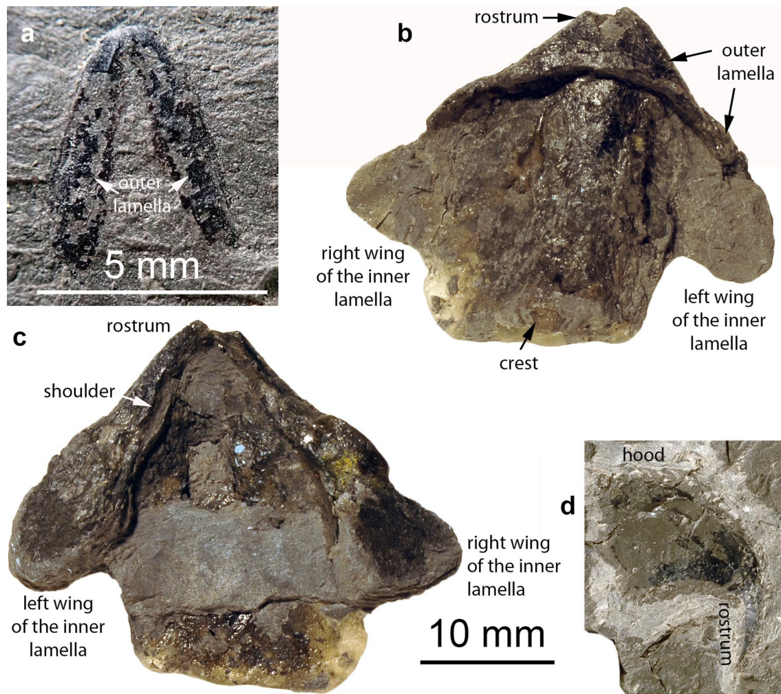
Fig. 2 Cephalopod jaws from the Opalinus Clay Formation of northern Switzerland. a PIMUZ 5942, upper jaw of an ammonoid ( Leioceras opalinum? ). b, c PIMUZ 6077, lower jaw of a megateuthid belemnite ( Acrocoelites conoideus? ); b ventral view, c dorsal view. d PIMUZ 6076, upper jaw of a megateuthid belemnite ( M. rhenana? ), seen laterally
