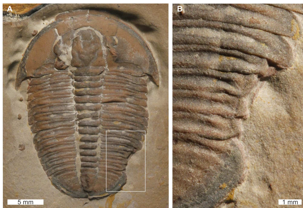
Figure 8 Elrathia kingii (Meek, 1870), UNSM PAL 729417, Wheeler Formation (Miaolingian Series, Drumian). (A) Complete specimen. (B) Close up of cicatrised, 'U'-shaped abnormality in box in (A). Full-size DOI: 10.7717/peerj.8453/fig-8
