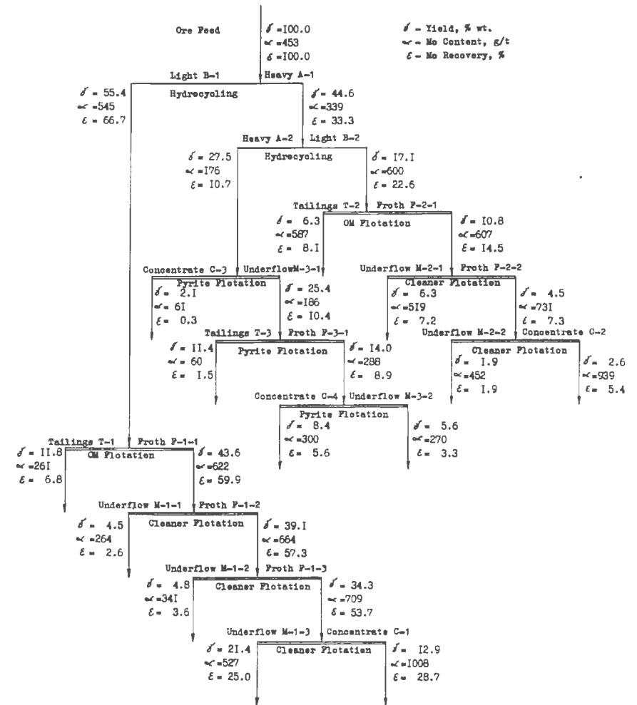
Fig. 2. Distribution of molybdenum on processing Toolse argillite
