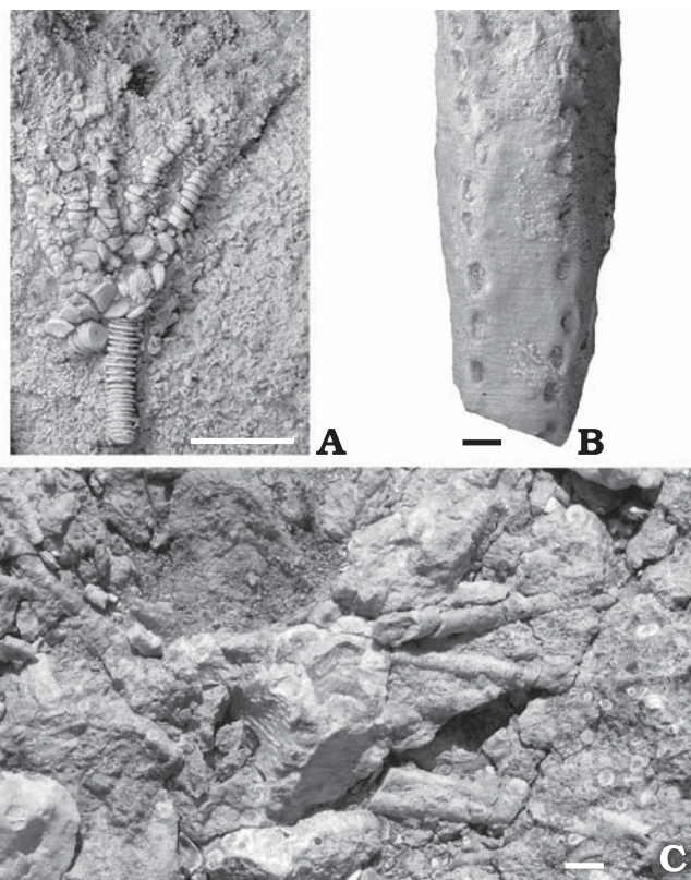
Fig. 6. Crinoids from the Silurian of Estonia, middle Äigu Beds, Kaugatuma Formation (Pridoli, Silurian), Kaugatuma Cliff. A. Cladida indet., TUG 1395-9, lateral view of badly disarticulated calyx. B. Enalloocrinus sp. holdfast, TUG 1395-39, column of Enalloocrinus holdfasts lacking the rhizoids. C. Field photograph of an uncollected in situ Enalloocrinus holdfast. Note wide, pentalobate lumen and long radices of holdfast. Scale bars 10 mm.
