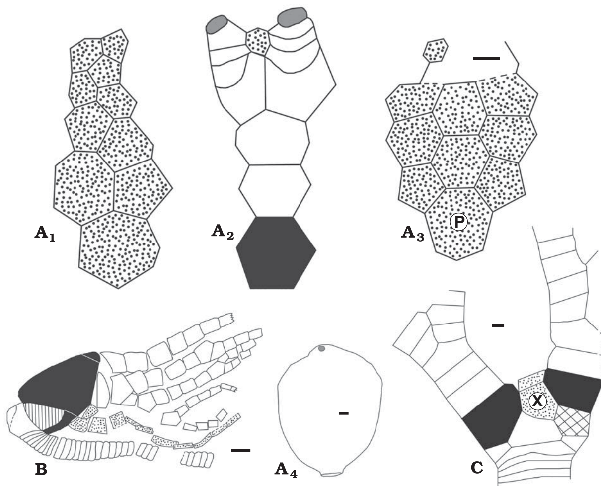
Fig. 4. Plate diagrams of Estonian crinoids. A. Saaremaacrinus estoniensis gen. et sp. nov., TUG 1395-3, middle Äigu Beds, Kaugatuma Formation (Pridoli), Kaugatuma Cliff. Normal interarray plating ( A_1 ), C-ray plating ( A_2 ), CD-interray plating ( A_3 ), and lateral outline of theca ( A_4 ). B. Calceocrinus baliticensis sp. nov., GIT 405-212, Juuru Stage (Llandovery), Heltermaa. D-ray view of crown. C. Protaxocrinus salteri ? (Angelin, 1878), TUG 1395-4, Ninase Member, Jaani Formation (Wenlock), Suuriku Cliff. Lateral outline. Plate designations: black, radial plate; ruled, inferradial plate; cross-ruled, radianal plate; stippled, interradyal plates or anal plates; P, primanal; X, anal X plate; grey, openings into theca. Scale bars 1 mm.
