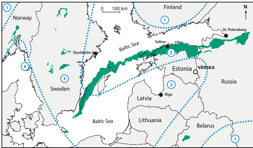
Fig. 1. Locality map showing the outcrop area of Ordovician rocks in the Baltic region (green) and schematic configuration of the Baltoscandian basin (after Männil 1966a and Nestor & Einasto 1997). 1, main land areas; 2, shallow-water Estonian shelf; 3, deeper-water Livonian basin and Central Baltoscandian facies belt; 4, deep shelf of the Scandian facies belt (modified after Toom et al. 2019a).
