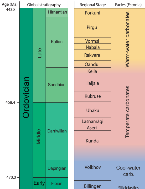
Fig. 2. Regional and international stratigraphy of the studied interval, showing transition from cool-water to warm-water carbonate deposits (modified after Toom et al. 2019a).
