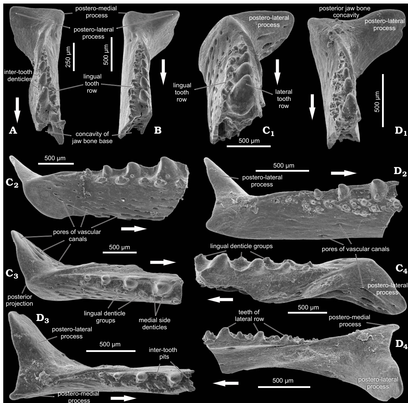
Fig. 7. Partial jaw bones of Early Devonian acanthodians from Ivanie-Zolote (A, B) and Zalizhchyky-1 (C, D). A, B. Podolicanthus zychi sp. nov. ZPAL P.14/12.4 (A) and ZPAL P.14/13.5 (B) in antero-occlusal view. C. Podolicanthus sp. 2. ZPAL P.14/7.3 in antero-occlusal (C 1 ), linguo-occlusal (C 2 ), occlusal (C 3 ), and lateral (C 4 ) views. D. Podolicanthus sp. 3. ZPAL P.14/12.12 in antero-occlusal (D 1 ), linguo-occlusal (D 2 ), occlusal (D 3 ), and lateral (D 4 ) view. Arrow indicates rostral direction.
