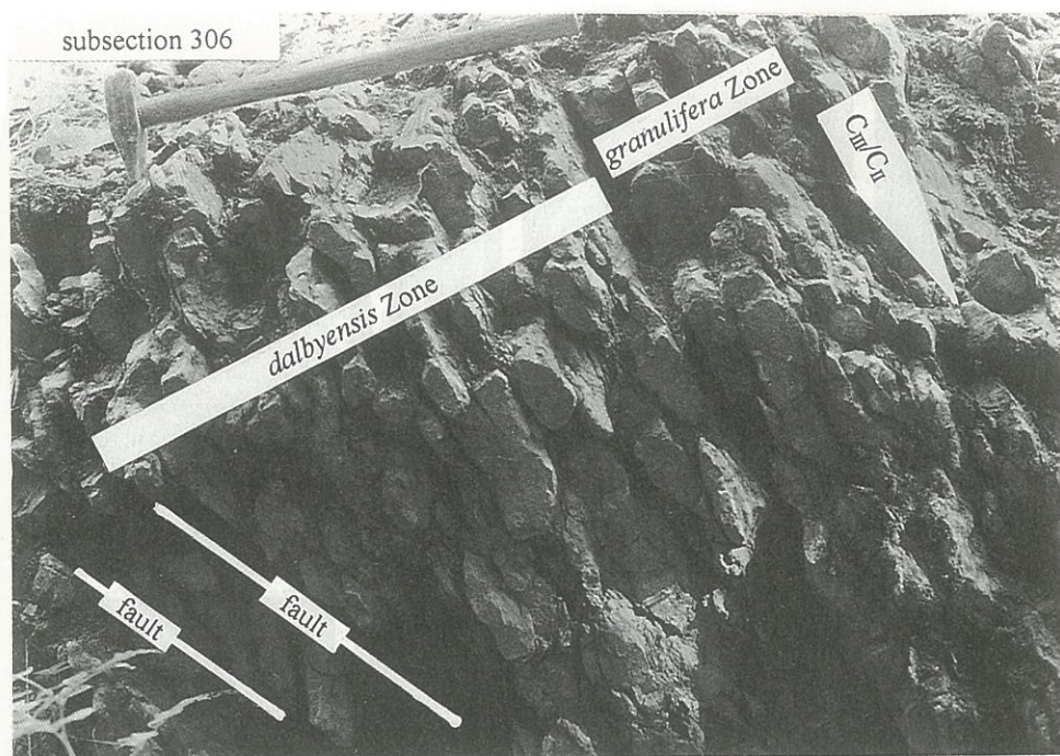
Fig. 4. Overthrusts and thickness of layers with chitinozoan biozones in the lowermost Idavere Substage in subsection 306 (see Fig. 1). C III , Kukruse Stage; C III , Idavere Substage of the Haljala Stage. Note the differences in the thickness of the dalbyensis Zone caused by faults.
