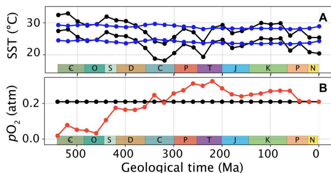
Fig. 1. SSTs and atmospheric p\text{O}_2 forcing. (A) Equatorial (10°S to 10°N) SSTs in the pre- and postwarming states (lower and upper curves, respectively) of the baseline and p\text{O}_2 (identical, black lines) and constant SST (blue lines) series of simulations. (B) Atmospheric p\text{O}_2 in baseline and constant SST (identical, black line) and p\text{O}_2 (red line) series of simulations. E, Cambrian; O, Ordovician; S, Silurian; D, Devonian; C, Carboniferous; P, Permian; T, Triassic; J, Jurassic; K, Cretaceous; P, Paleogene; N, Neogene.
