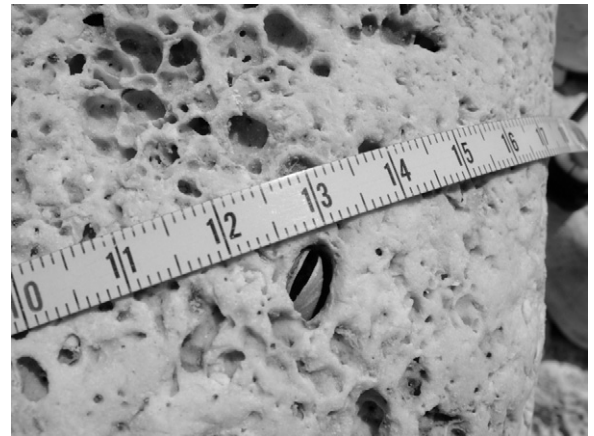
Fig. 11. Gastrochaenolites with its producer inside.
