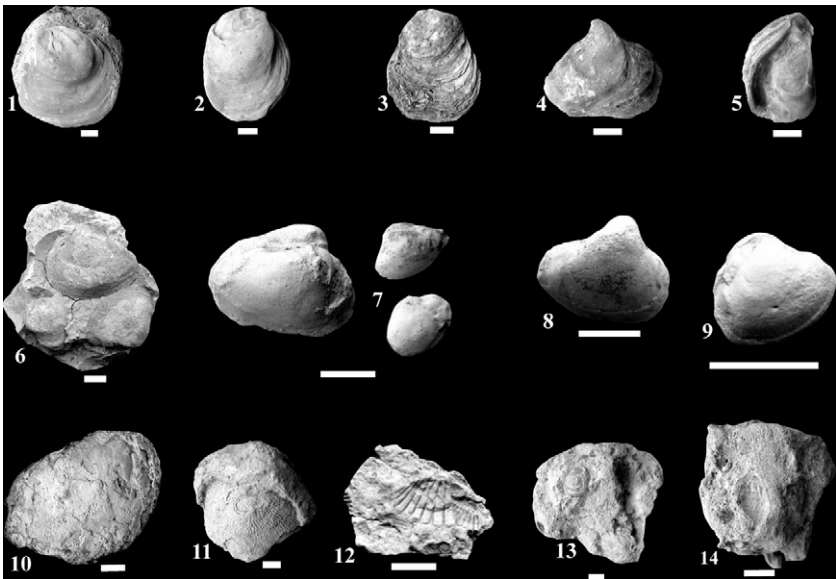
Fig. 7. Well-preserved marine macrofossils at Alcitepe Formation (Scale: 1 cm). Fig. 7. Macrofossiles marins bien conservés de la Formation Alcitepe (échelle = 1 cm).
