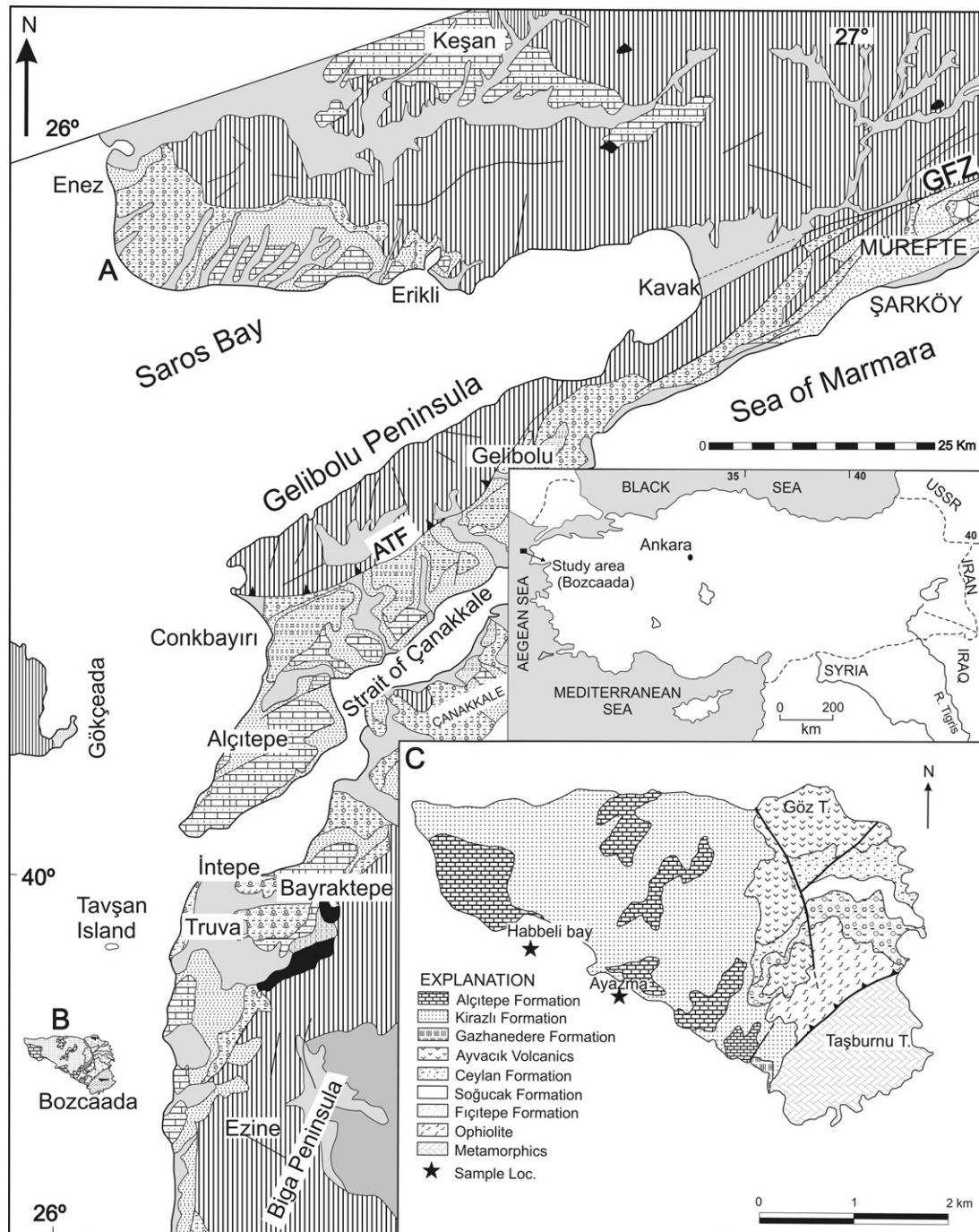
Fig. 1. A, B. Geological map of the northeastern Aegean region (modified from Sakinç and Yaltırak, 2005 ). C. Close up view of the study area (modified from Temel and Çiftçi, 2002 ).
