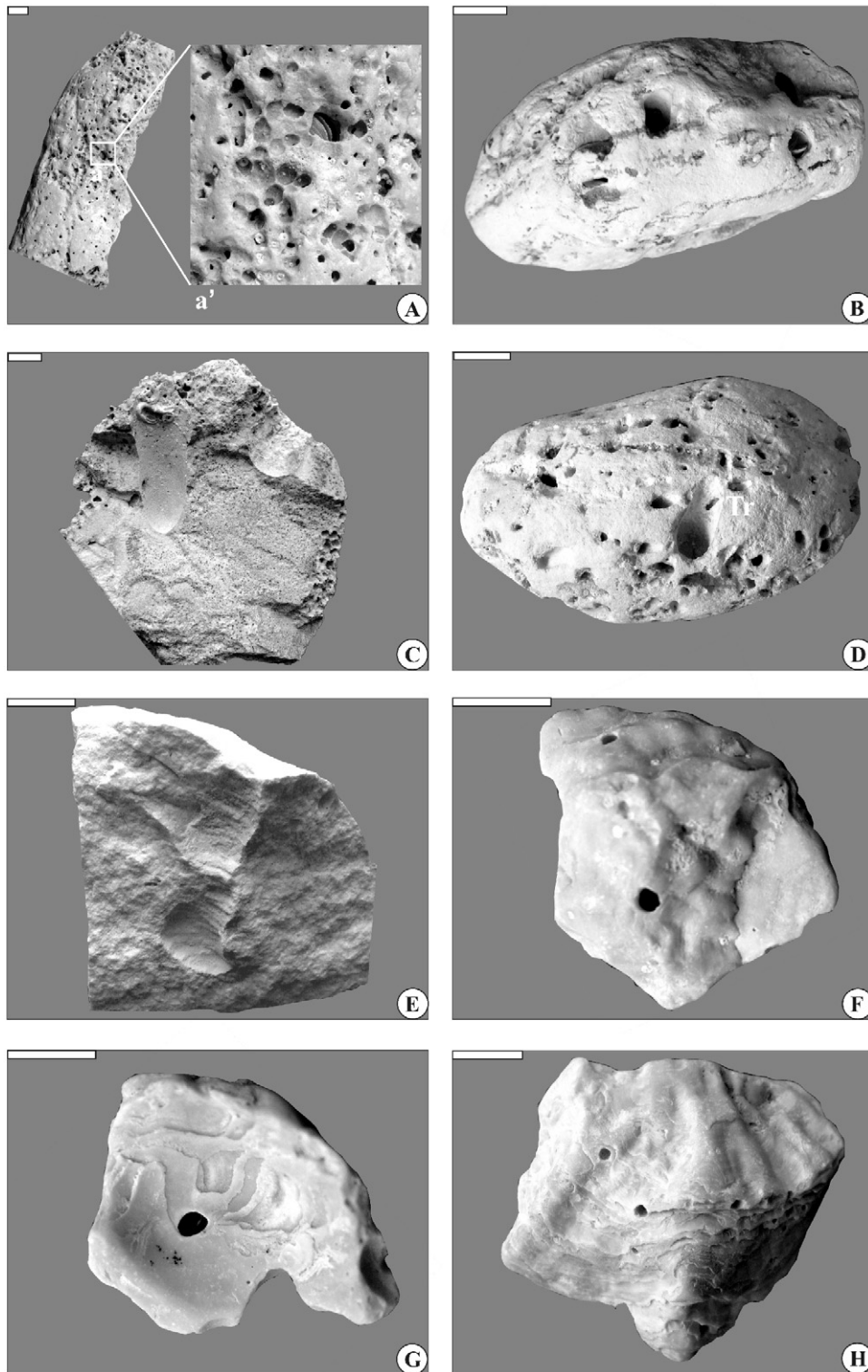
Plate 3. Images of inferred bivalve borings and drill holes-duraphagous scars from the Alçıtepe limestone boulders and shells (All scales: 1 cm). A. Gastrochaenolites isp. B. Gastrochaenolites lapidicus . C. Gastrochaenolites torpedo . D. Gastrochaenolites torpedo with Trypanites isp. E. Phrixichnus isp. F. Oichnus isp. G. Oichnus isp. H. Oichnus isp.
