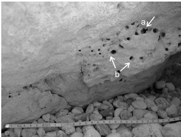
Fig. 9. View of Gastrochaenolites torpedo (a), Gastrochaenolites lapidicus (b).
