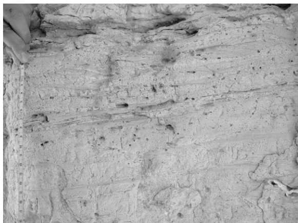
Fig. 6. Shallow marine-shore face cross lamination, Alcítepe Formation.
