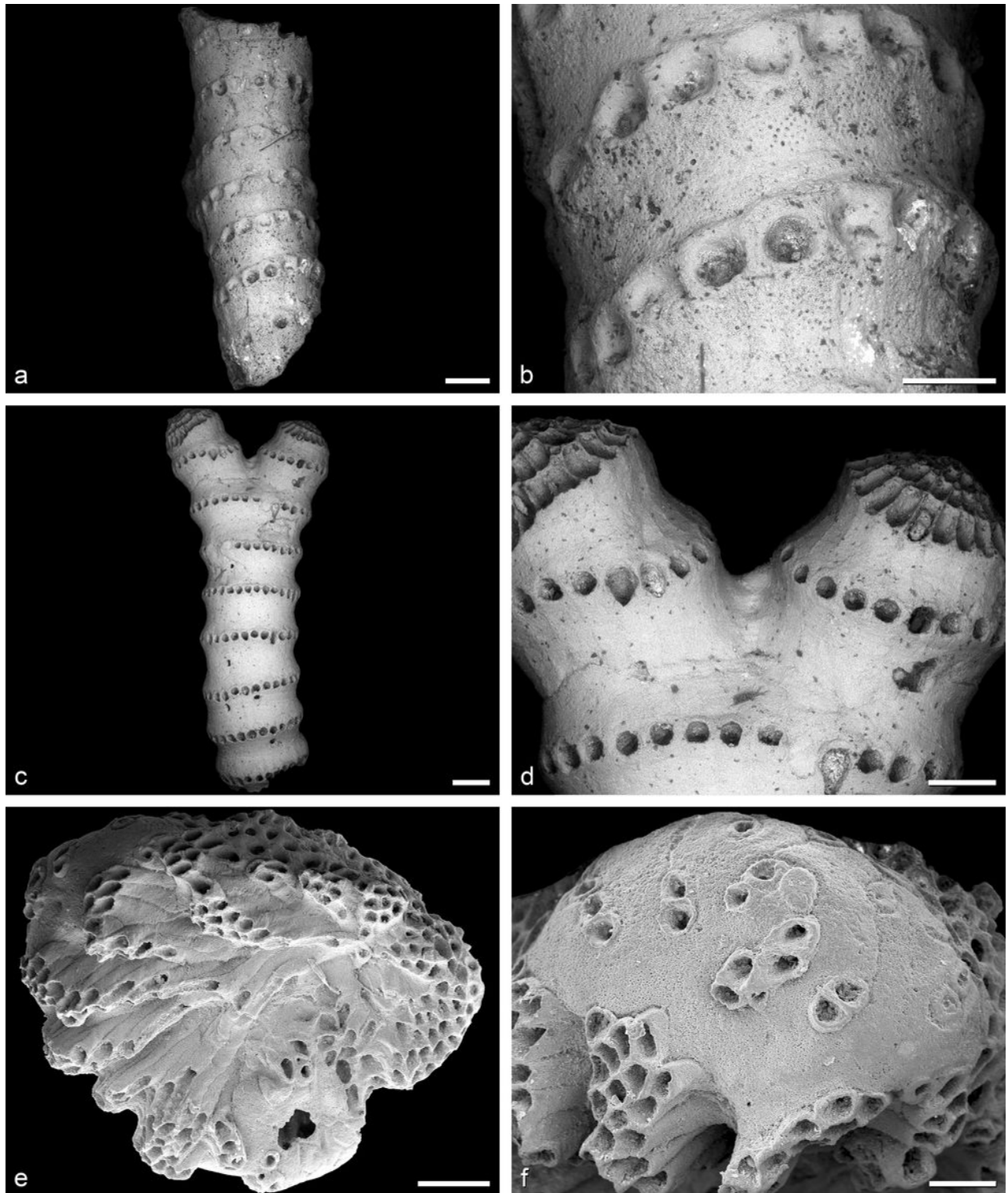
Figure 24: a-b Spiropora (?) ingens VOIGT, 1924, neotype, SMF 24360, middle Santonian ( Gonioteuthis westfalica belemnite Zone), abandoned quarry of the former iron-ore mine of Bülten-Adenstedt near Ilsede-Groß Bülten, Lower Saxony, Germany. c-d Spiropora suecica VOIGT & FLOR, 1970, holotype, SMF 24351, late Campanian, Hemmingslycke near Kristianstad, Skåne län, Sweden. e-f Fascigera fasciculus VOIGT, 1967, holotype, SMF 24214, late Maastrichtian, Hemmoor, Lower Saxony, Germany. Scale bars: a, c 1 mm; b, d-e 500 µm; f 250 µm.
