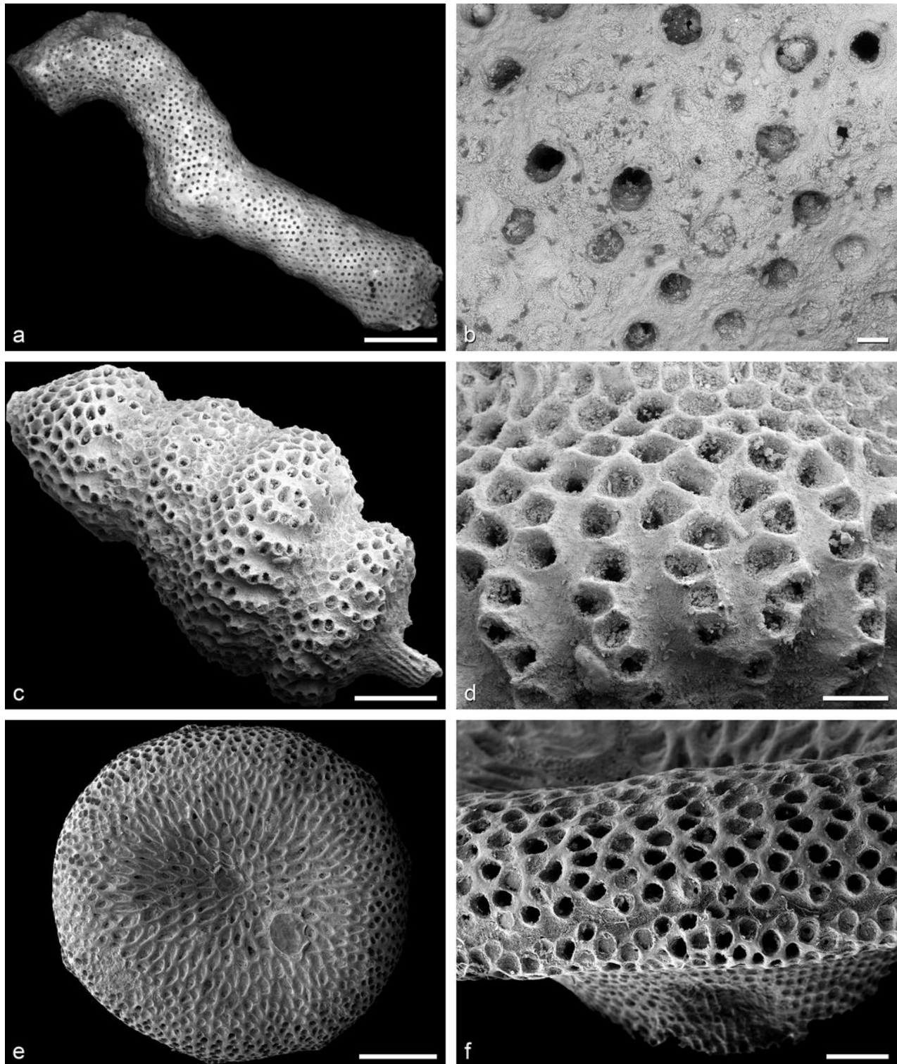
Figure 8: a-b Pachyteichopora punctata VOIGT, 1978, holotype, SMF 24683, late Campanian ( Belemnitella mucronata belemnite Zone), Båstad, Skåne län, Sweden. c-d Stylodefranciopora turris VOIGT & VÁVRA, 2006, holotype, SMF 26248, early Maastrichtian, Saturn pit near Krons Moor, Schleswig-Holstein, Germany. e-f Amphimarssoniella klaumanni VOIGT, 1974, holotype, SMF 24533, early Cenomanian ( Neostlingoceras carcitense ammonite Zone), Kasenberg, Rauen Quarry in Mülheim an der Ruhr-Broich, North Rhine-Westphalia, Germany. Scale bars: a, e 2.5 mm; c 1 mm; f 500 µm; d 250 µm; b 100 µm.
