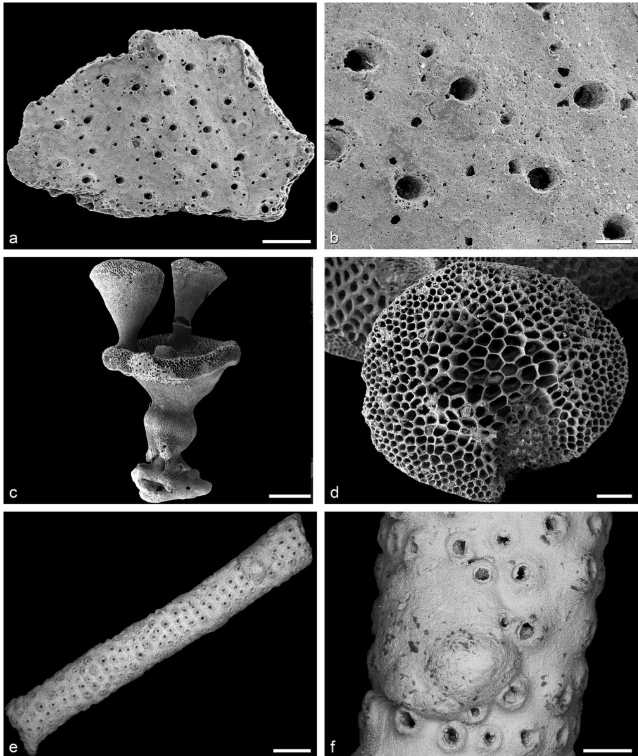
Figure 7: a-b Cryptoglena adspersa (MARSSON, 1887), neotype, SMF 24920, early Maastrichtian, Island of Rügen, Mecklenburg-Vorpommern, Germany. c-d Marssoniella cenomana VOIGT, 1974, holotype, SMF 24549, early Cenomanian ( Neostlingoceras carcitanense ammonite Zone), Kassenberg, Rauen Quarry in Mülheim an der Ruhr-Broich, North Rhine-Westphalia, Germany. e-f Pachyteichopora bugei VOIGT, 1978, holotype, SMF 24690, Coniacian, probably Tours, Centre-Val de Loire, France. Scale bars: c 2.5 mm; e 1 mm; a, d 500 µm; f 250 µm; b 100 µm.
