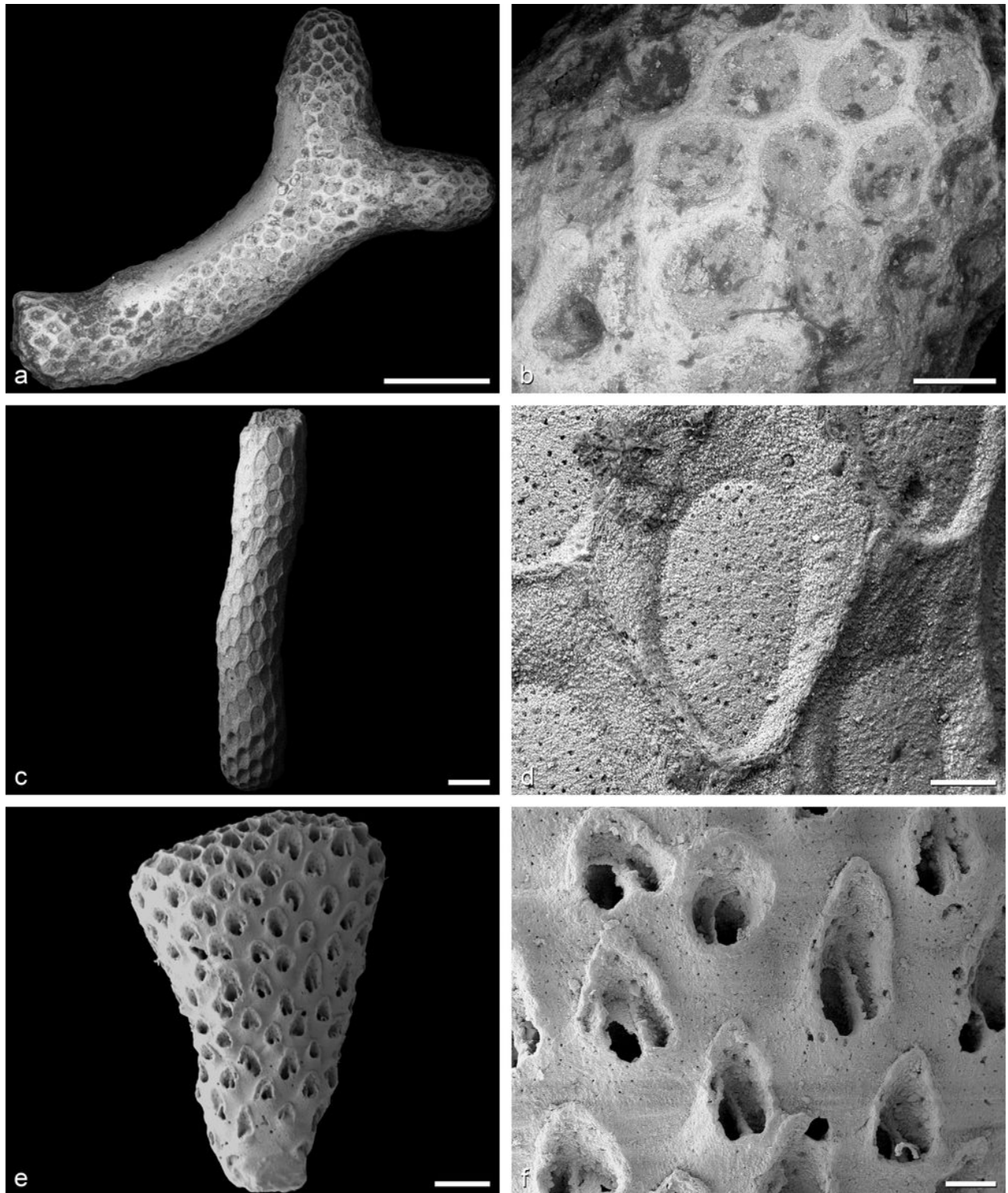
Figure 23: a-b Filicea cincta VOIGT, 1924, neotype, SMF 24449, late Santonian, Burgberg near Gehrden, Lower Saxony, Germany. c-d Filicea velata (HAGENOW, 1839), neotype, SMF 26395, early Maastrichtian, Island of Rügen, Mecklenburg-Vorpommern, Germany. e-f Septocea septifera VOIGT, 1995, holotype, SMF 26106, early Maastrichtian, Stubbenkammer on the Island of Rügen, Mecklenburg-Vorpommern, Germany. Scale bars: a 2.5 mm; c 1 mm; e 500 µm; b 250 µm; d, f 100 µm.
