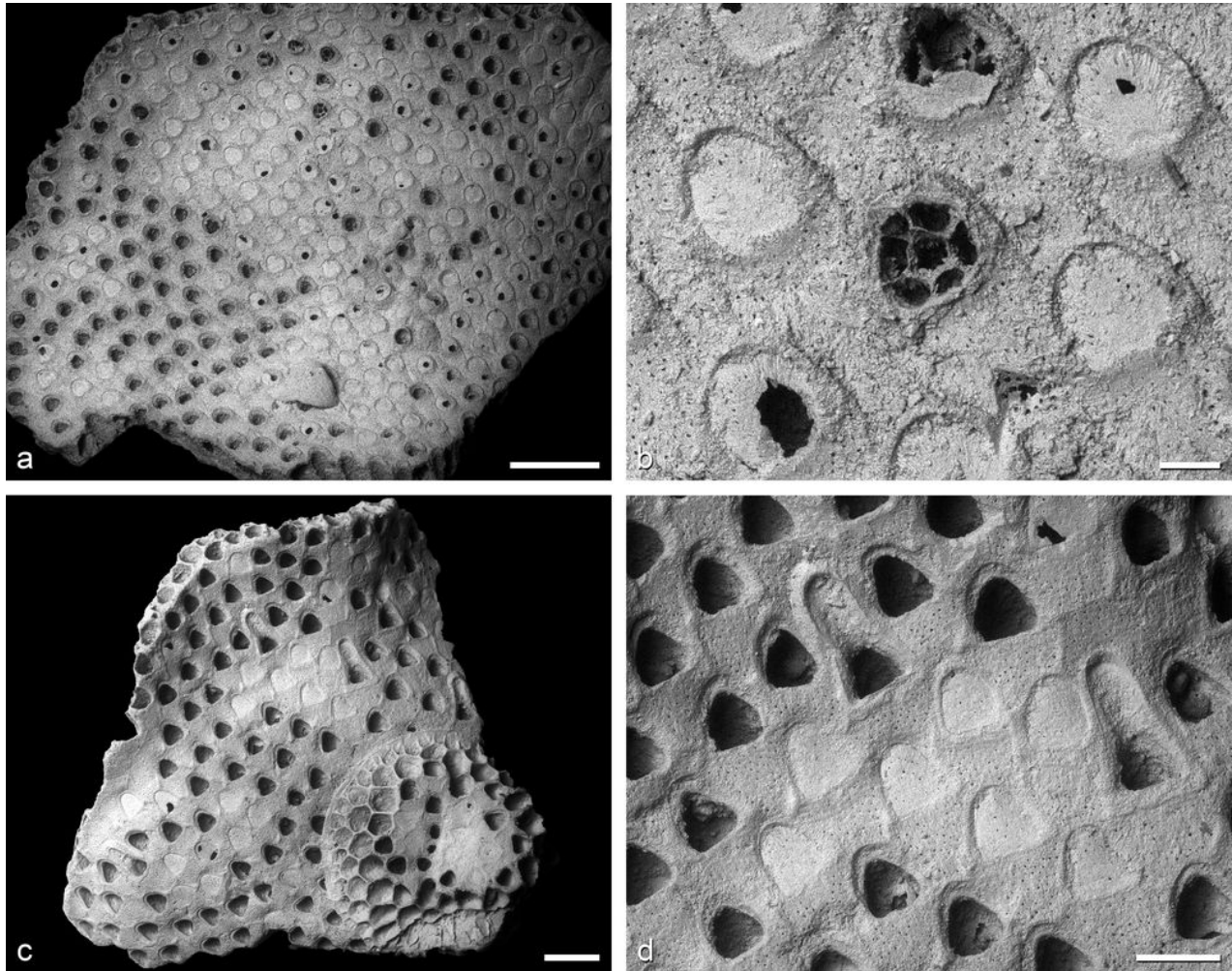
Figure 14: a-b Reptomultelea reedi TAYLOR, 1994, holotype, SMF 26537, late Cenomanian, Saint-Calais, Sarthe, Pays de la Loire, France. c-d Reptomultelea scanica TAYLOR, 1994, holotype, SMF 26540, early Campanian ( Belemnelloamax mammillatus belemnite Zone), Karlshamn, Blekinge län, Sweden. Scale bars: a 1 mm; c 500 \mu m; d 250 \mu m; b 100 \mu m.
