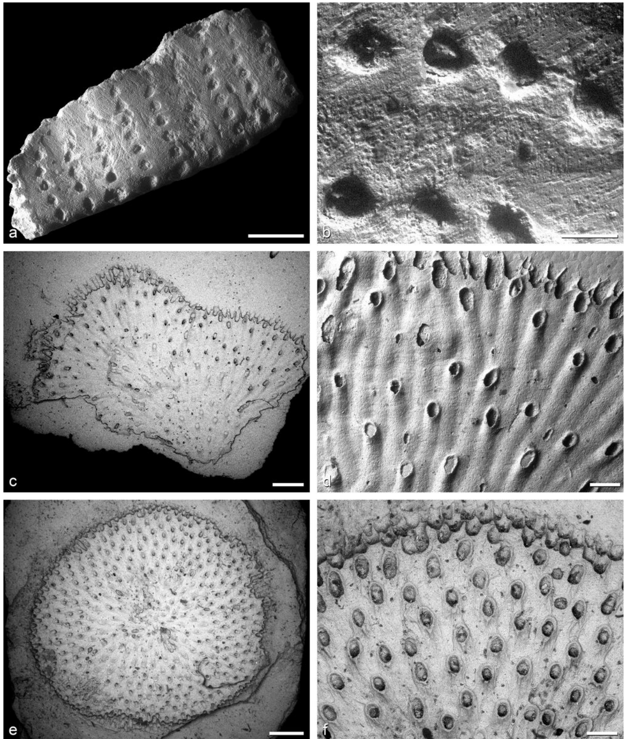
Figure 21: a-b Reptoclausula wolffi VOIGT, 1924, neotype, SMF 26433, Santonian, Burgberg west of Gehrden, Lower Saxony, Germany. c-d Diplosolen pavonius VOIGT, 1929, neotype, SMF 26391, early Maastrichtian, Island of Rügen, Mecklenburg-Vorpommern, Germany. e-f Plagioecia disciformis (HAGENOW, 1839), neotype, SMF 26388, early Maastrichtian, Island of Rügen, Mecklenburg-Vorpommern, Germany. Scale bars: c-d 1 mm; a 500 µm; d, f 250 µm; b 100 µm.
