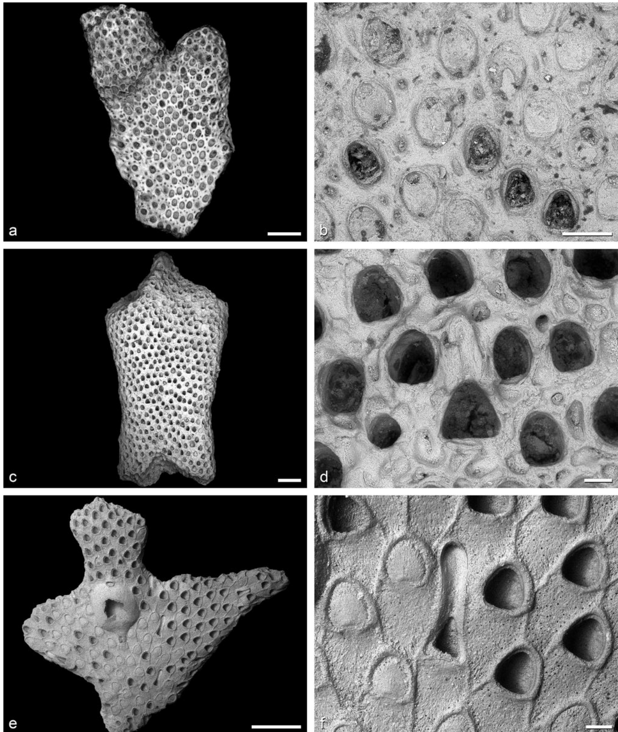
Figure 9: a-b Biforicula acuminata (VOIGT, 1973), holotype, SMF 26436, middle Santonian ( Gonioteuthis westfalica belemnite Zone), abandoned Barbara pit near Lengede-Barbecke, Lower Saxony, Germany. c-d Biforicula ? nodulifera (VOIGT, 1924), neotype, SMF 26436, late Santonian, Burgberg west of Gehrden, Lower Saxony, Germany. e-f Elea elegantula TAYLOR, 1994, holotype, SMF 26499, early Cenomanian ( Neostlingoceras carcitanense ammonite Zone), Kassenberg, Rauhen Quarry in Mülheim an der Ruhr-Broich, North Rhine-Westphalia, Germany. Scale bars: a, c, e 1 mm; b 250 µm; d, f 100 µm.
