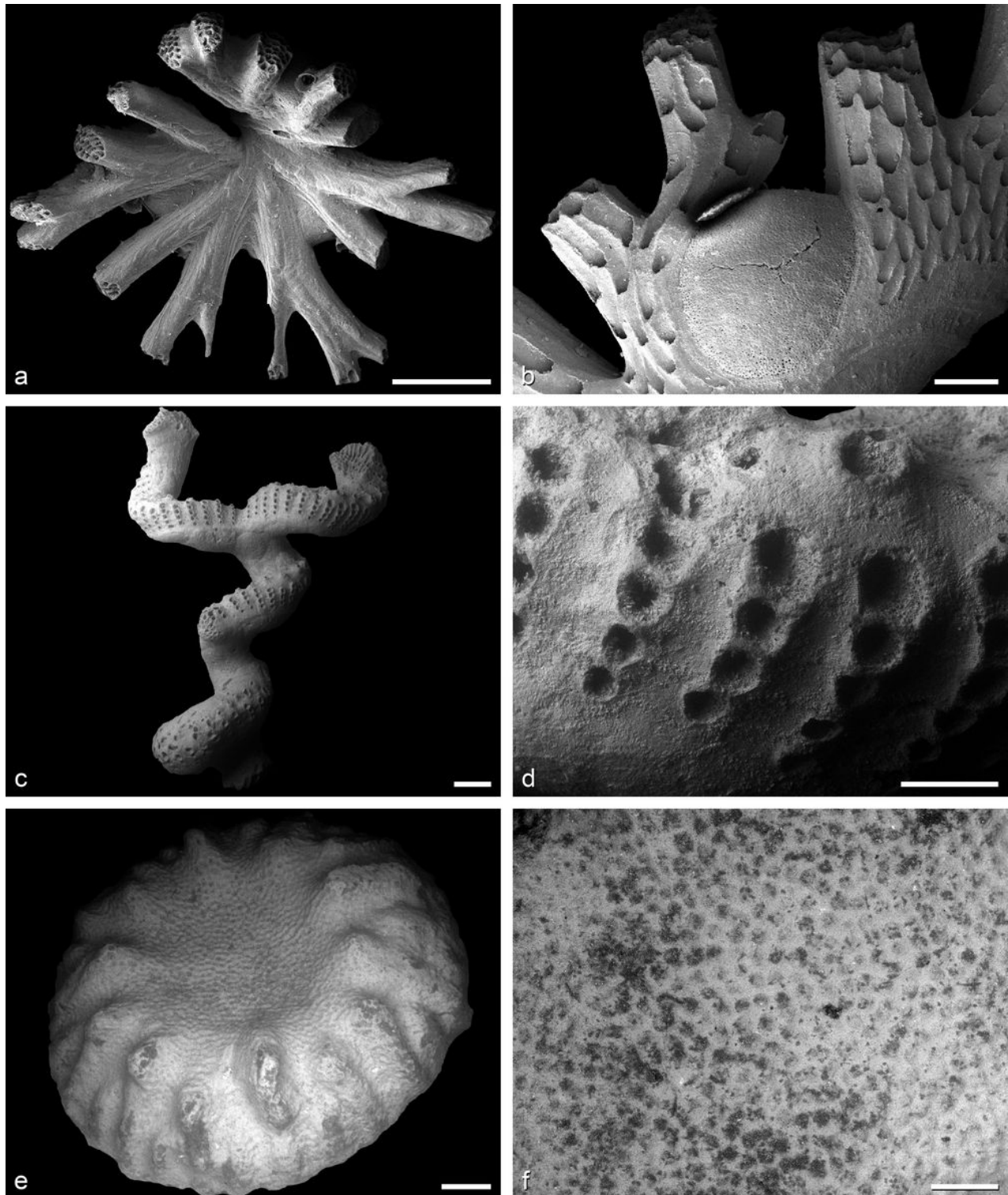
Figure 4: a-b Discotruncatulipora corbis FLOR, 1975, holotype, SMF 26460, early Cenomanian ( Neostlingoceras carcitense ammonite Zone), Kassenberg, Rauen Quarry in Mülheim an der Ruhr-Broich, North Rhine-Westphalia, Germany. c-d Heterocrisina candelabrum VOIGT, 1987, holotype, SMF 25495, late Maastrichtian ( Belemnitella junior belemnite Zone), Sint-Pietersberg near Maastricht, Limburg, Netherlands. e-f Infundibulipora huckriedei VOIGT, 1977, holotype, SMF 24033, Campanian or Maastrichtian, southern side of the valley of "Kischk" and "Kemunu" northwest of the village Kemunu in the Darmanu Mountains northwest of Kerman, Kerman Province, Iran. Scale bars: a, c, e 1 mm; f 500 µm; b, d 250 µm.
