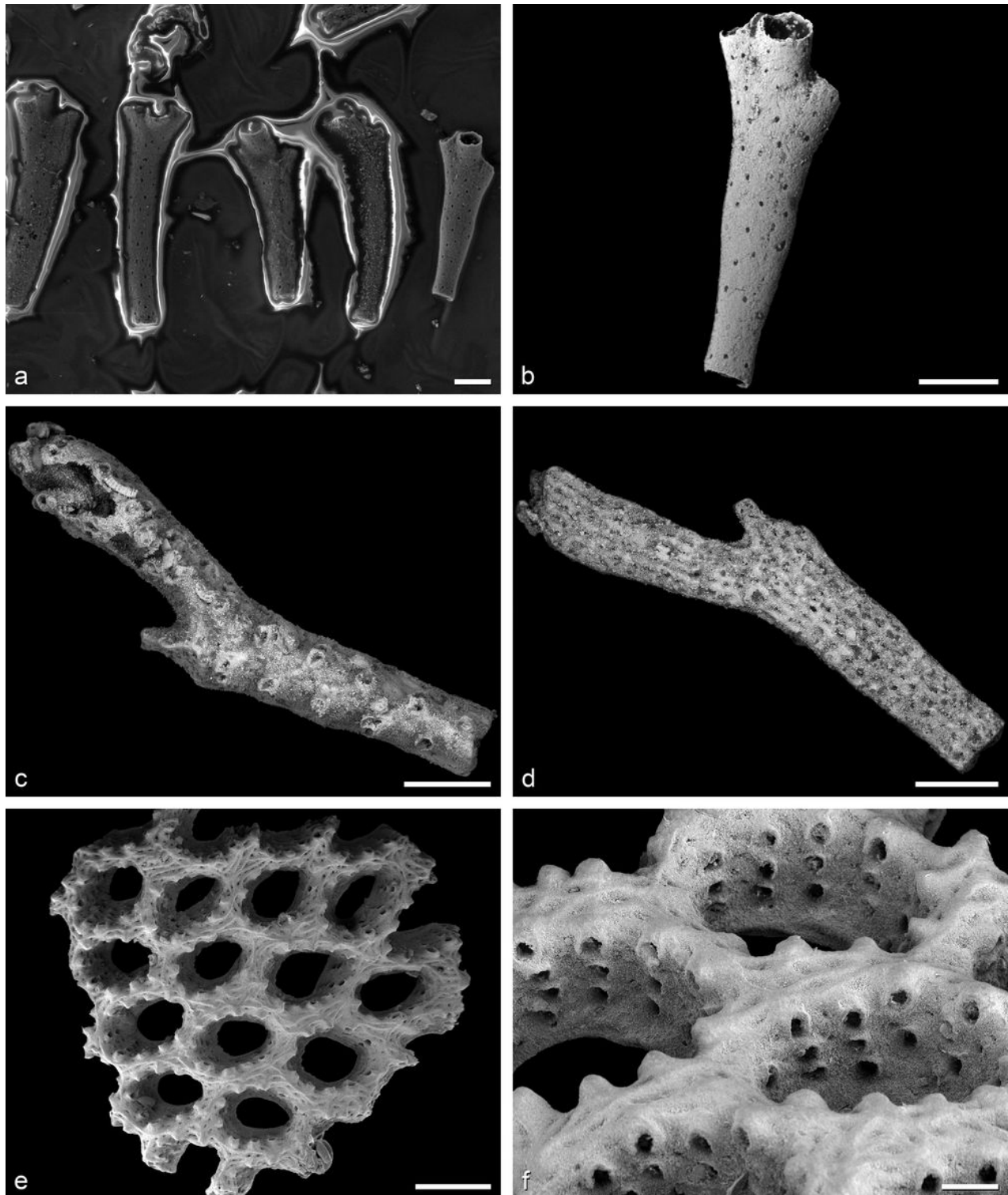
Figure 2: a-b Crisidia lagaaiji VOIGT, 1987, holotype, SMF 25533, Danian, Ciply in the municipality Mons, Wallonia, Belgium. c-d Polyascosoecia pseudolichenoides VOIGT, 1987, SMF 25553, Danian, Ciply in the municipality Mons, Wallonia. e-f Reteporidae georgiknetschi VOIGT, 1984, holotype, SMF 25297, early Maastrichtian ( Belemnite junior belemnite Zone), Blom Quarry near Terblijt in the municipality Valkenburg aan de Geul, Limburg, Netherlands. Scale bars: e 1 mm; c-d 500 \mu m; f 250 \mu m; a-b 100 \mu m.
