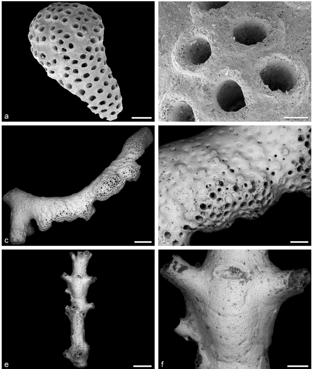
Figure 30: a-b Ramofilisparsa walteri VOIGT, 1989, holotype, SMF 25807, early Cenomanian ( Neostlingoceras carci-tanense ammonite Zone), Kassenberg, Rauen Quarry in Mülheim an der Ruhr-Broich, North Rhine-Westphalia, Germany. c-d Retecavella broodi VOIGT, 1987, holotype, SMF 25519, Danian, Curfs Quarry near Berg, Valkenburg aan de Geul, Limburg municipality, Netherlands. e-f Spirentalophora brandesi VOIGT & FLOR, 1970, holotype, SMF 24404, middle Santonian ( Gonioteuthis westfalica belemnite Zone), abandoned quarry of the former iron-ore mine of Bültens-Adenstedt near Ilsede-Groß Bültens, Lower Saxony, Germany. Scale bars: c, e 1 mm; a 500 \mu m; d, f 250 \mu m; b 100 \mu m.
