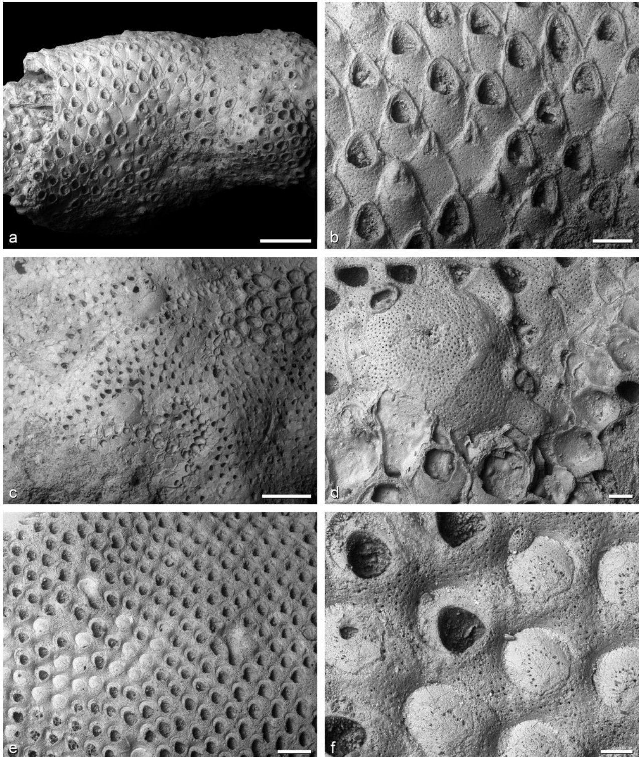
Figure 13: a-b Reptomultelea convexa TAYLOR, 1994, holotype, SMF 26524, probably Turonian, Chenu, Pays de la Loire, France. c-d Reptomultelea parvula TAYLOR, 1994, holotype, SMF 26531, early Cenomanian ( Neostlingoceras carcitanense ammonite Zone), Kassenberg, Rauen Quarry in Mülheim an der Ruhr-Broich, North Rhine-Westphalia, Germany. e-f Reptomultelea pegma TAYLOR, 1994, holotype, SMF 26532, early Cenomanian ( Neostlingoceras carcitanense ammonite Zone), Kassenberg, Rauen Quarry in Mülheim an der Ruhr-Broich, North Rhine-Westphalia, Germany.
