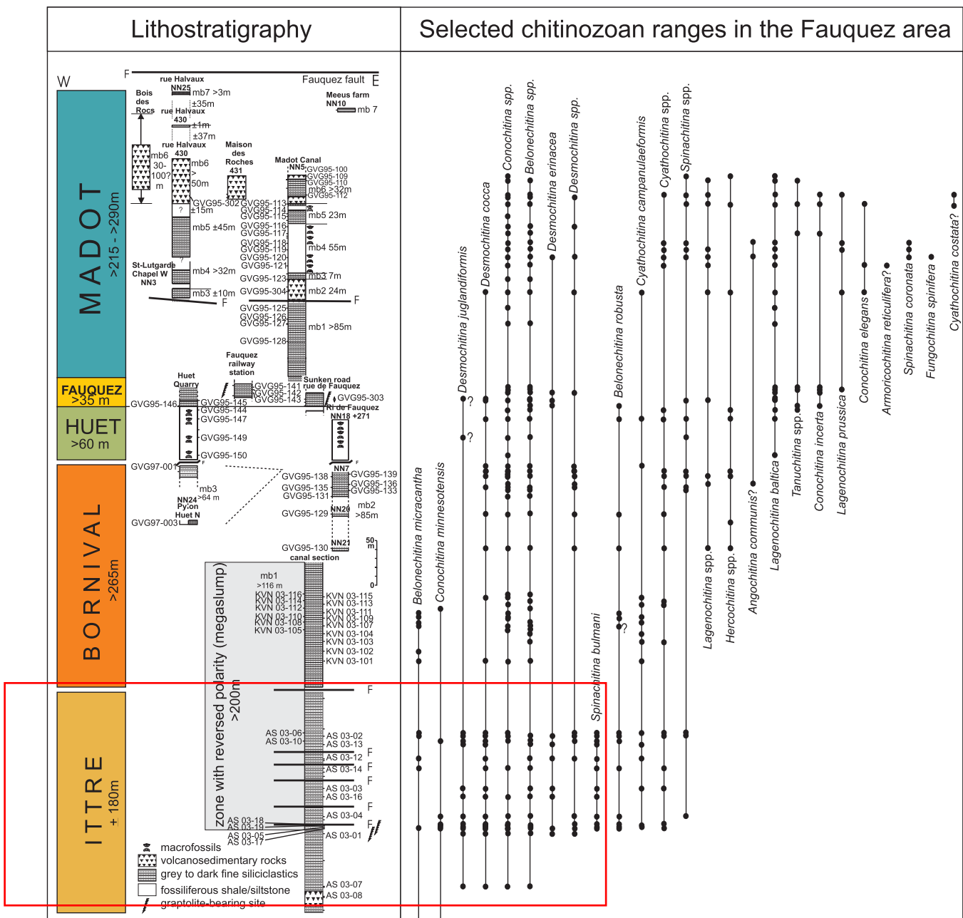
Figure 2. Lithostratigraphy, position of the samples, and chitinozoan ranges in the investigated formations. Lithologs modified from Van Grootel et al. (1998), except for the Ittre Formation and the lower member of the Bornival Formation.
