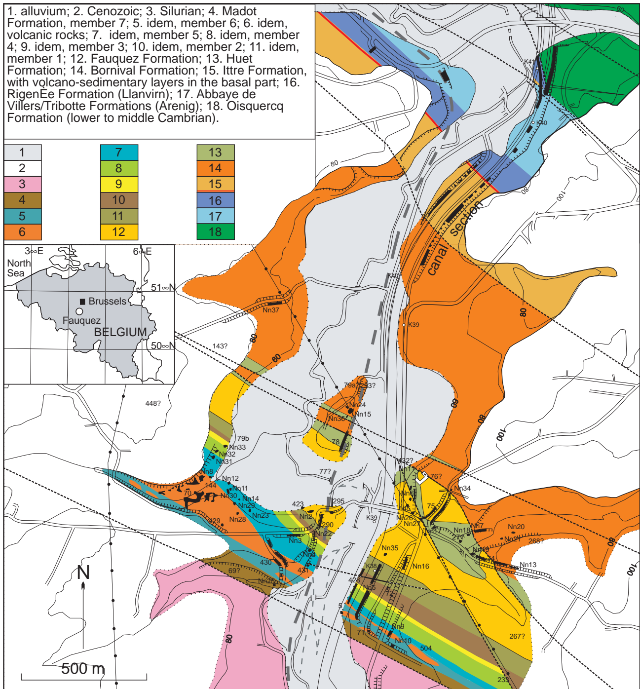
Figure 1. Geological map of the Lower Palaeozoic of the Fauquez and Asquempont areas with location of the outcrops. Compiled and modified from Debacker (2001) and Verniers et al. (this volume) for the southern part, and Debacker (2001) and Debacker et al. (2003) for the northern part.
