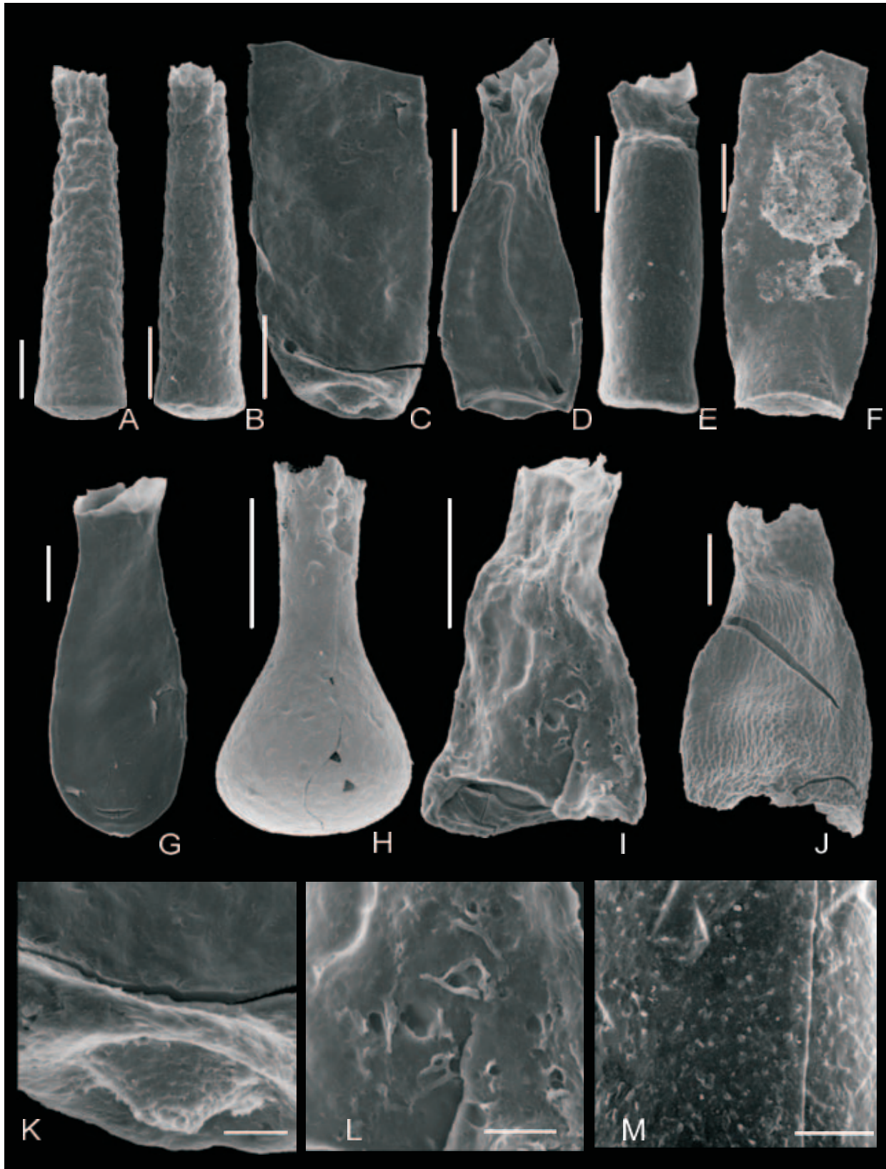
Plate 3. SEM photographs of chitinozoans from the Fauquez and Madot formations. Scale bars on complete specimen photographs represent 50 \mu\text{m} . Scale bars on detail photographs represent 10 \mu\text{m} .
