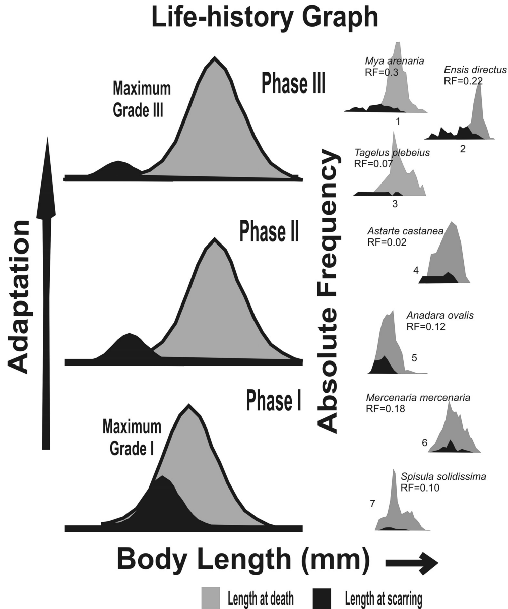
FIGURE 7. The model shows (left column) how species' adaptation allows it to reduce frequencies of severe damages with time (i.e., from Phase I to Phase III). In addition to it, the model also shows how death due to scarring is minimized by moving away from the frequency distribution of length at scarring (see text). The right column presents many examples of these distributions, redrawn from Alexander and Dietl (2001).
