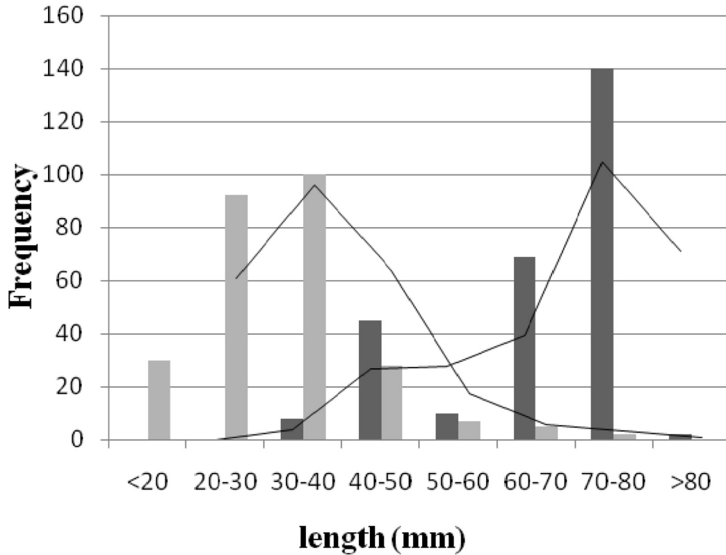
FIGURE 5. The graph shows absolute frequency distribution of 'length at death' and 'length at the incidence of scarring' on bivalve shells. Note marked differences in absolute frequency distributions of these two lengths. Presence of non-random distribution of 'length at death' indicates that the samples are not winnowed from the actual habitat of the living bivalves.
