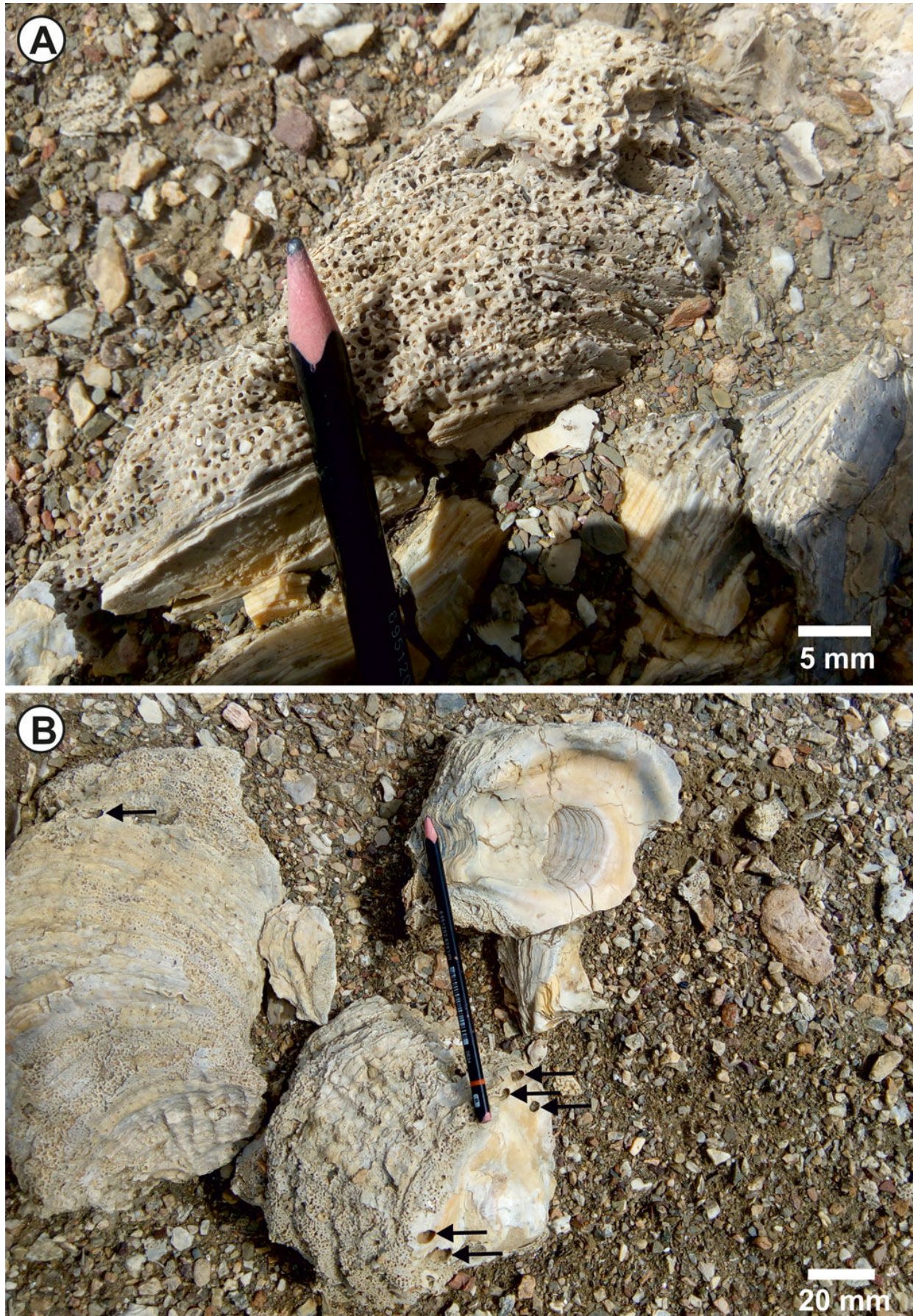
Figure 2: (A) abundant Entobia cf. geometrica borings in an O. lamellosa shell; (B) O. lamellosa shells bored by both Entobia and Gastrochaenolites (arrows indicate Gastrochaenolites burrows).
