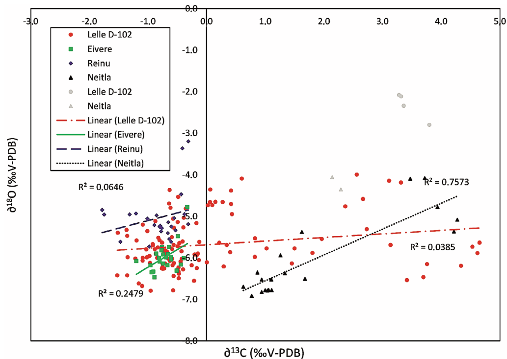
Fig. 4. Oxygen vs carbon isotopic composition measured from bulk carbonate material in the studied stratigraphic units. The light grey data points mark the likely altered samples from the Kamariku Formation and were not taken into account when calculating R^2 .
