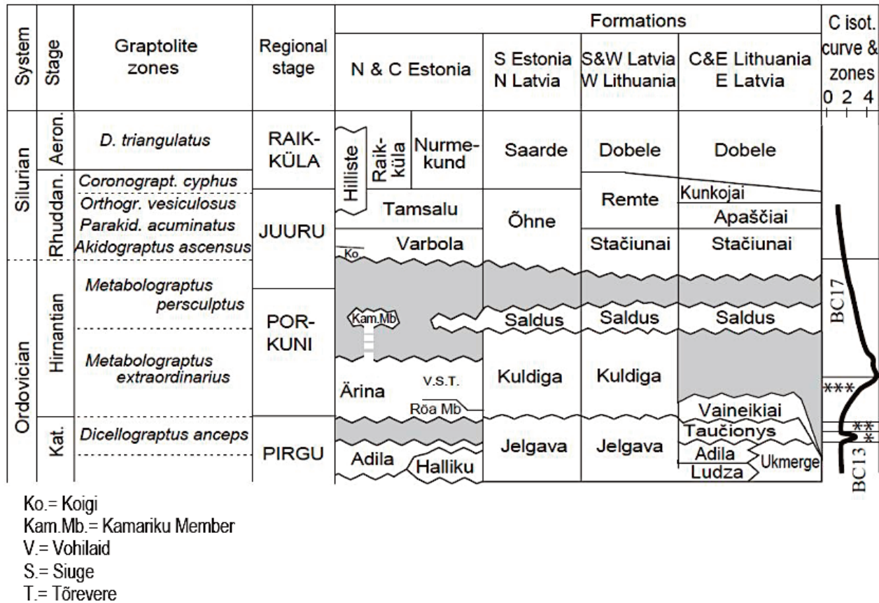
Fig. 2. The latest Ordovician and early Silurian stratigraphy of the Baltic region (Truuver et al. 2021).
