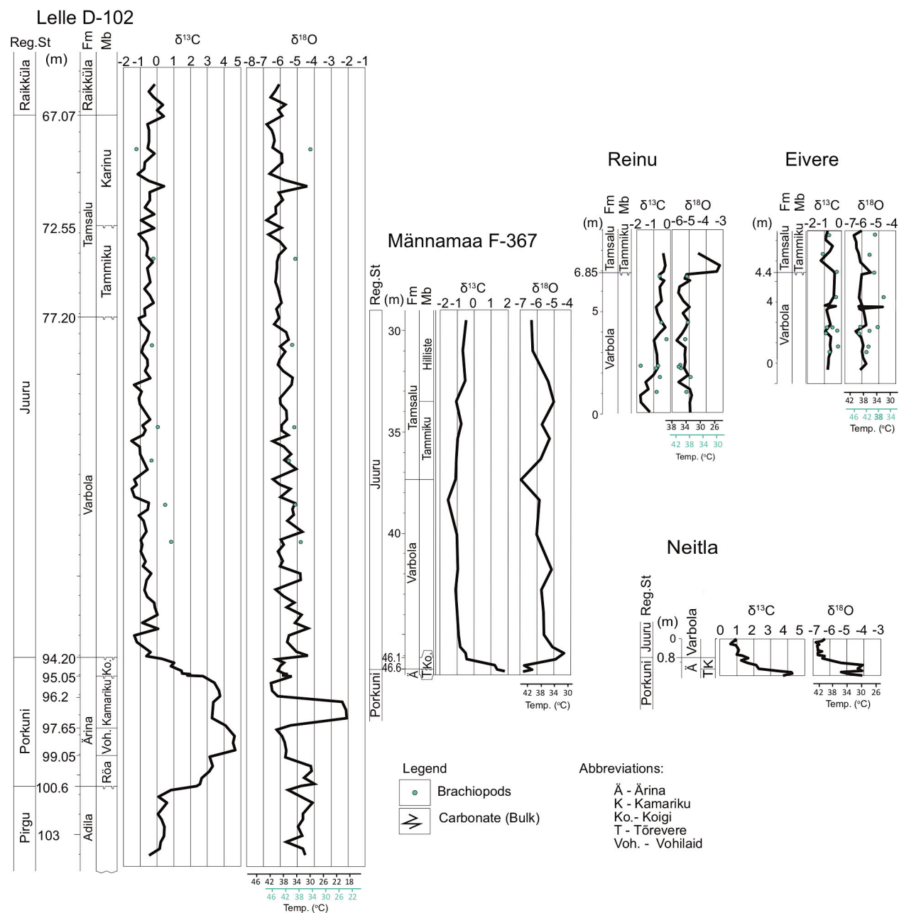
Fig. 3. The \delta^{13}\text{C} and \delta^{18}\text{O} curves of the studied sections. Circles show isotope values of brachiopod shells. Temperatures were calculated from bulk rock data by the formula of Kim & O’Neil (1997), assuming the possible preservation of the original marine carbonate isotopic composition formed in sea water with the \delta^{18}\text{O} value of -1\text{‰} . The temperature scale in black shows palaeotemperatures from bulk carbonate samples. As a different formula (Brand et al. 2019) was used for calculating palaeotemperature values from brachiopods, the respective temperature scale is shown in blue. Abbreviations: Reg.St, Regional Stage; Fm, Formation; Mb, Member.
